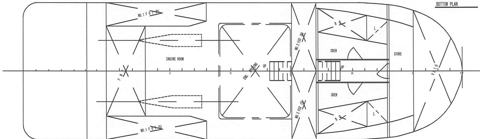
BOTTOM PLAN
